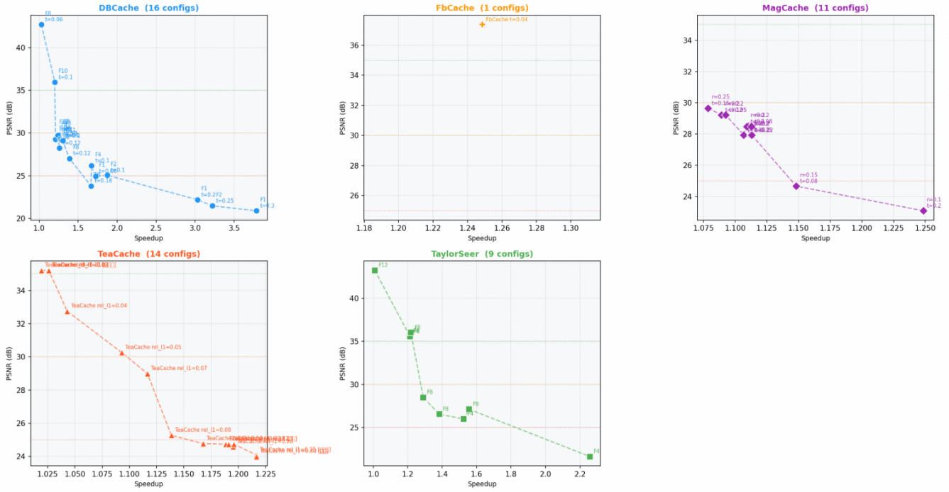
Cache Type Parameter Sweep: PSNR vs Speedup (each point = one config; line connects configs of same type ordered by speedup)
