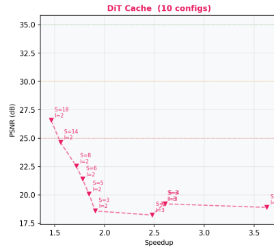
Cache Type Parameter Sweep: PSNR vs Speedup (each point = one config; line connects configs of same type ordered by speedup)
