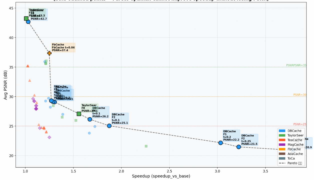
Cache Scheme Pareto Frontier (bold-outlined points = Pareto optimal: cannot improve speedup without losing PSNR)
