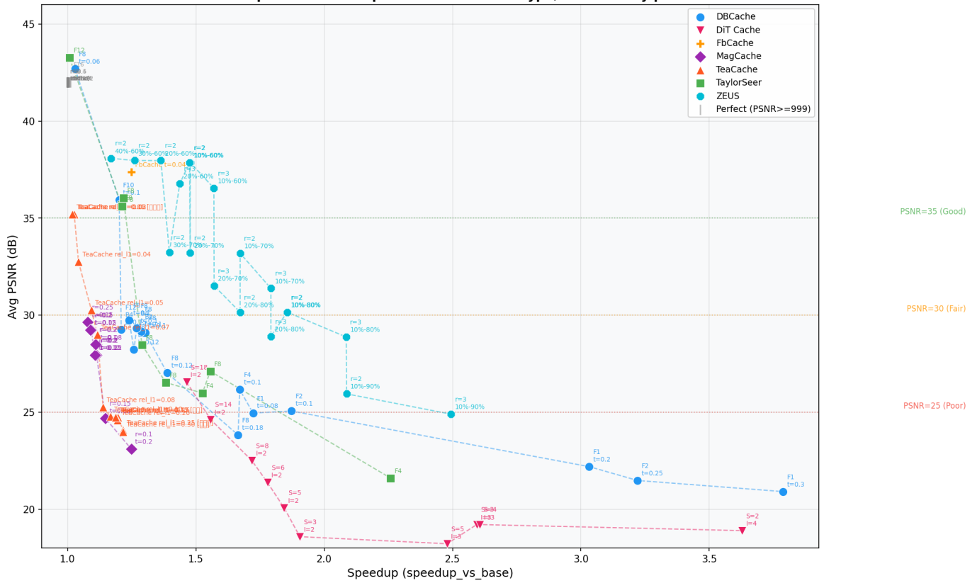
Cache Scheme Pareto Frontier (bold-outlined points = Pareto optimal: cannot improve speedup without losing PSNR)
