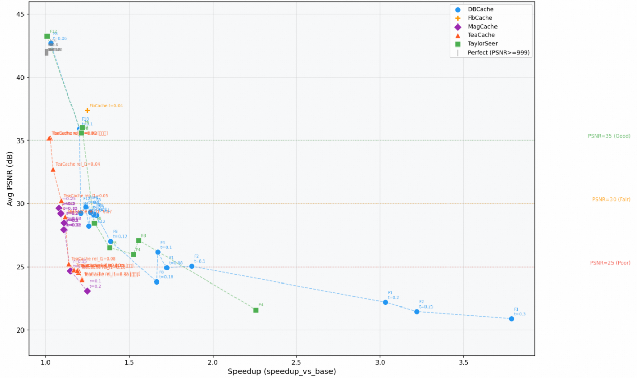
Cache Scheme PSNR vs Speedup (adp_1 + adp_2 + adp_3) Dashed line = parameter sweep within same cache type; labels = key params
